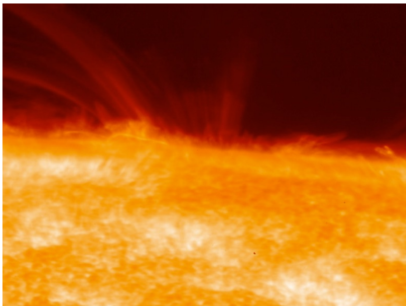
FIGURE 1. Top: large-scale solar magnetism. The eleven-year magnetic solar cycle (#21 – 22) observed in the chromosphere through the H\alpha spectral line (full solar discs), and historical sunspot-number record (Credits: NOAA/Zürich/RDC/CNRS/INSU/Ondrejov Observatory/HAO). Bottom: local and global solar magnetic dynamics. The rapidly-evolving small-scale magnetic carpet, spicules and sunspot arches imaged near the limb in the lower chromosphere through the CaH spectral line (Credits: SOT/Hinode/JAXA/NASA).
