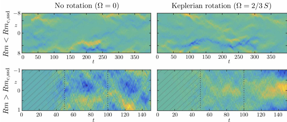
FIGURE 35. Space-time diagrams showing the evolution of a large-scale dynamo magnetic field \overline{B}_y(z, t) in local Cartesian shearing box numerical simulations of dynamo action in the presence of forced, non-helical small-scale turbulence, shear \mathbf{U}_S = -Sx \mathbf{e}_y , with or without global rotation \boldsymbol{\Omega} = \Omega \mathbf{e}_z . Top row: simulations at Rm lower than Rm_{c,ssd} for small-scale dynamo action (adapted from Squire & Bhattacharjee 2015c). Bottom row: simulations at Rm larger than Rm_{c,ssd} . Hatches indicate the phase of small-scale dynamo growth (adapted from Squire & Bhattacharjee 2015b, 2016). Left: simulations with shear, but no rotation. Right: simulations with Keplerian rotation, \Omega = (2/3)S . The box size (L_x, L_y, L_z) is (1, 1, 16) in the top-row calculations with no small-scale dynamo, and (1, 4, 2) in the more computationally demanding bottom-row calculations with a small-scale dynamo. All four simulations are in a regime of Re and Rm that is linearly and nonlinearly stable to hydrodynamic shear instabilities and MHD instabilities such as the magnetorotational instability. In all cases, the turbulence is forced at a scale \ell_0 = L_x/3 much smaller than that at which the large-scale dynamo fields develop, and has a turnover rate u_{rms}/\ell_0 comparable to the shearing rate S .
