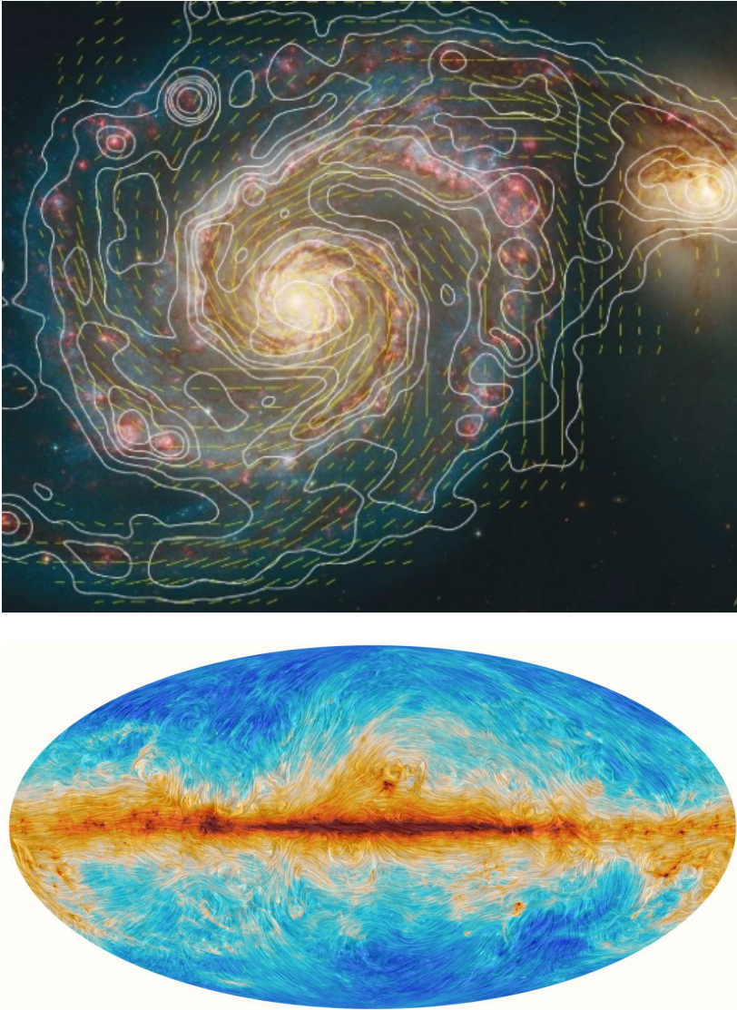
FIGURE 3. Top: large-scale spiral magnetic structure (line segments) of the M51 galaxy established from radio observations of polarised synchrotron emission by cosmic rays (Credits: MPIfR Bonn and Hubble Heritage Team. Graphics: Sterne and Weltraum). Bottom: map of the microwave galactic dust emission convolved with galactic magnetic-field lines reconstructed from polarisation maps of the dust emission (Credits: M. A. Miville-Deschênes/CNRS/ESA/Planck collaboration).
