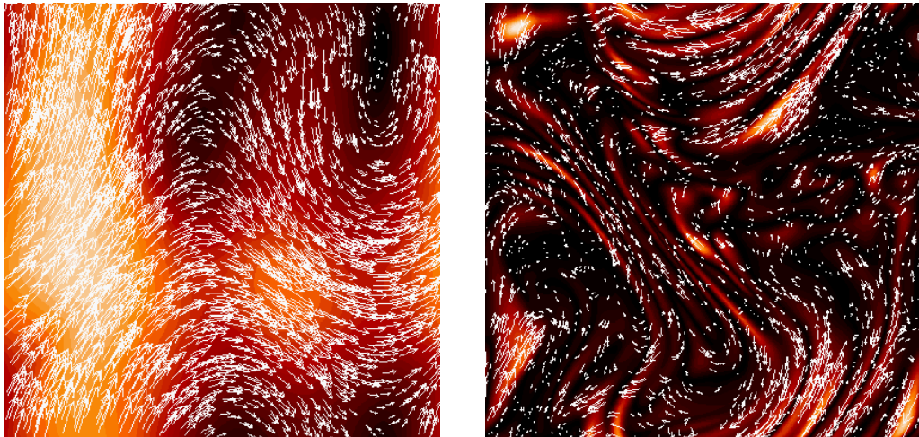
FIGURE 14. Left: 2D snapshot of |\mathbf{u}| in a 3D simulation of non-helical, homogeneous, isotropic smooth random flow forced at the box scale \ell_0 for Re = 1 ( \ell_\nu = \ell_0 ). Right: snapshot of the strength |\mathbf{B}| of the kinematic dynamo magnetic field generated by this flow for Rm = Pm = 1250 , and corresponding magnetic field directions (arrows). The field in this large- Pm regime has a strongly folded geometric structure: it is almost uniform along itself, but reverses on the very fine scale \ell_\eta/\ell_0 \sim Pm^{-1/2} , \sim 0.03 in that example. The brighter regions correspond to large field strengths (adapted from Schekochihin et al. 2004c ).
