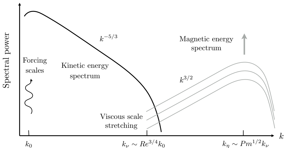
FIGURE 20. Evolution of the magnetic energy spectrum in the kinematic, diffusive large- Pm regime. The shape of the magnetic spectrum is now fixed in time and peaks at the resistive scale k_\eta , but the magnetic energy continues to grow exponentially.
