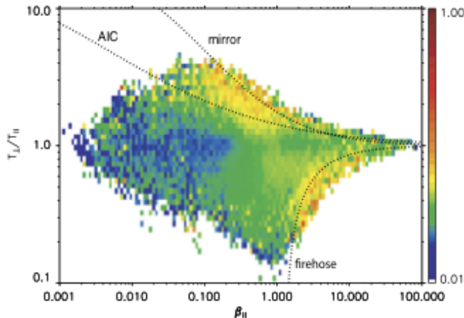
FIGURE 47. Example of statistics of ion temperature anisotropy versus \beta_i in the solar wind (Bale et al. 2009). Most recorded events at \beta_i > 1 are confined into a region of parameter space seemingly delimited by the linear threshold of the mirror ( \Delta_i = 1/\beta_i ) and firehose ( \Delta_i = -2/\beta_i ) instabilities (dotted lines). The AIC line corresponds to a fixed small ion-cyclotron instability iso-growth-rate line.
