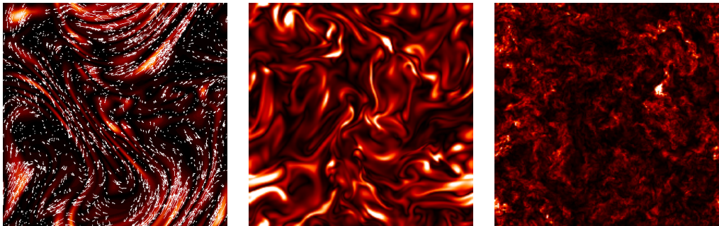
FIGURE 16. 2D snapshots of the strength |B| of the kinematic dynamo magnetic field for 3D simulations of non-helical, homogeneous, isotropic turbulence forced at the box scale. Left: Pm = Rm = 1250 , Re = 1 . Centre: Pm = 1 , Re = Rm = 440 . Right: Pm = 0.07 , Rm = 430 , Re = 6200 (because this particular simulation uses hyperviscous dissipation only, the kinetic Reynolds number in this case is defined using an effective viscosity determined statistically from the simulation data). Note the very different magnetic field structures between the Pm = 1 and Pm = 0.07 cases, despite Rm being essentially the same in both simulations (adapted from Schekochihin et al. 2007).
