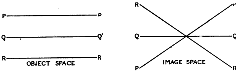
Fig. 2. Negative Lens.
