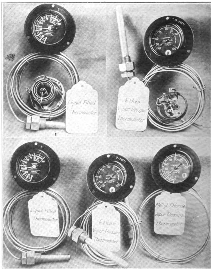
FIG. 24. Liquid and Vapor Pressure Thermometers
